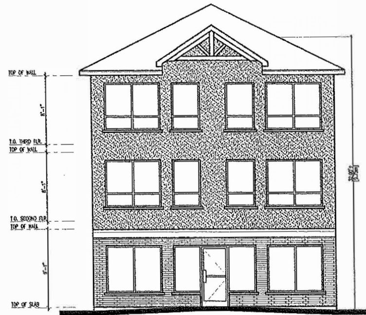
FRONT (SOUTH) ELEVATION
