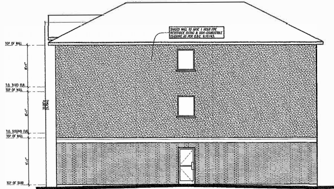
RIGHT (EAST) ELEVATION
