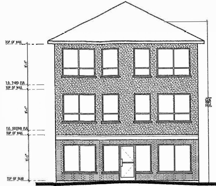
REAR (NORTH) ELEVATION
